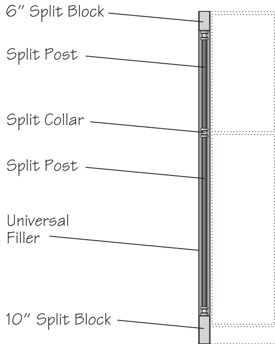
Tall Cabinet
