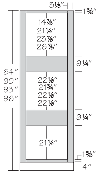
Single Oven Cabinet 4 Butt Doors*
