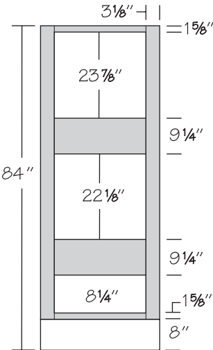
Universal Design Oven Cabinet
