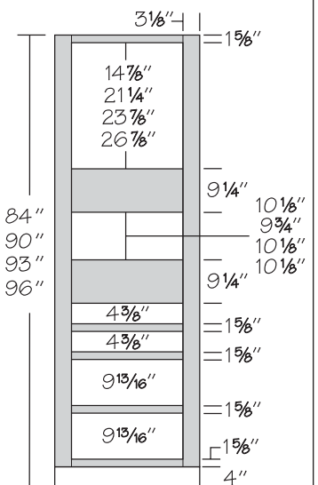
Single Oven Cabinet 2 Butt Doors, 4 Drawers*
