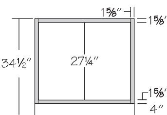
Vanity Full-Height Base Cabinet
